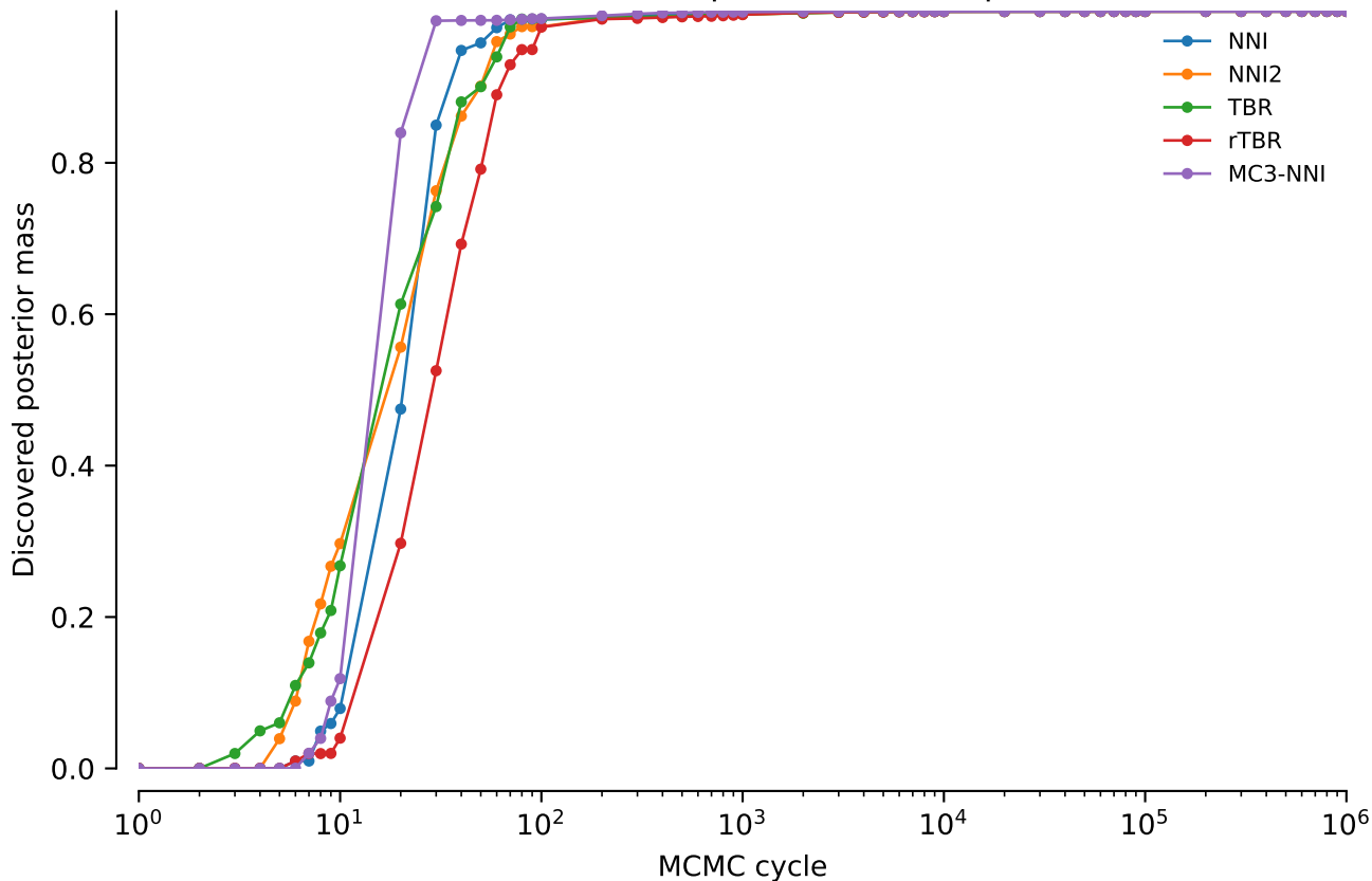
vert.nd2.tw0: Discovered posterior mass: power = 0.05
