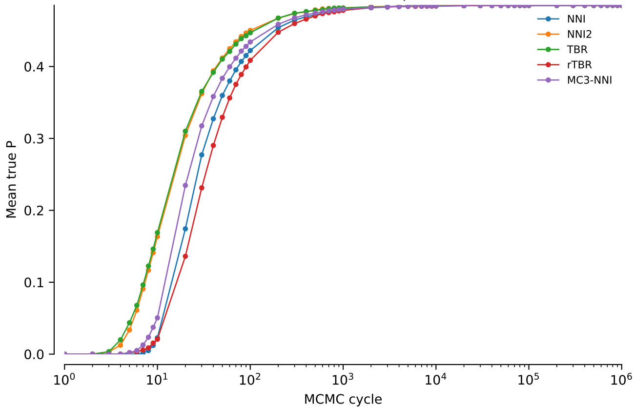
vert.nd2.tw0: Mean true P: power = 0.1
