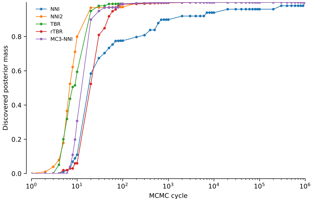
vert.nd2.tw0: Discovered posterior mass: power = 0.2
