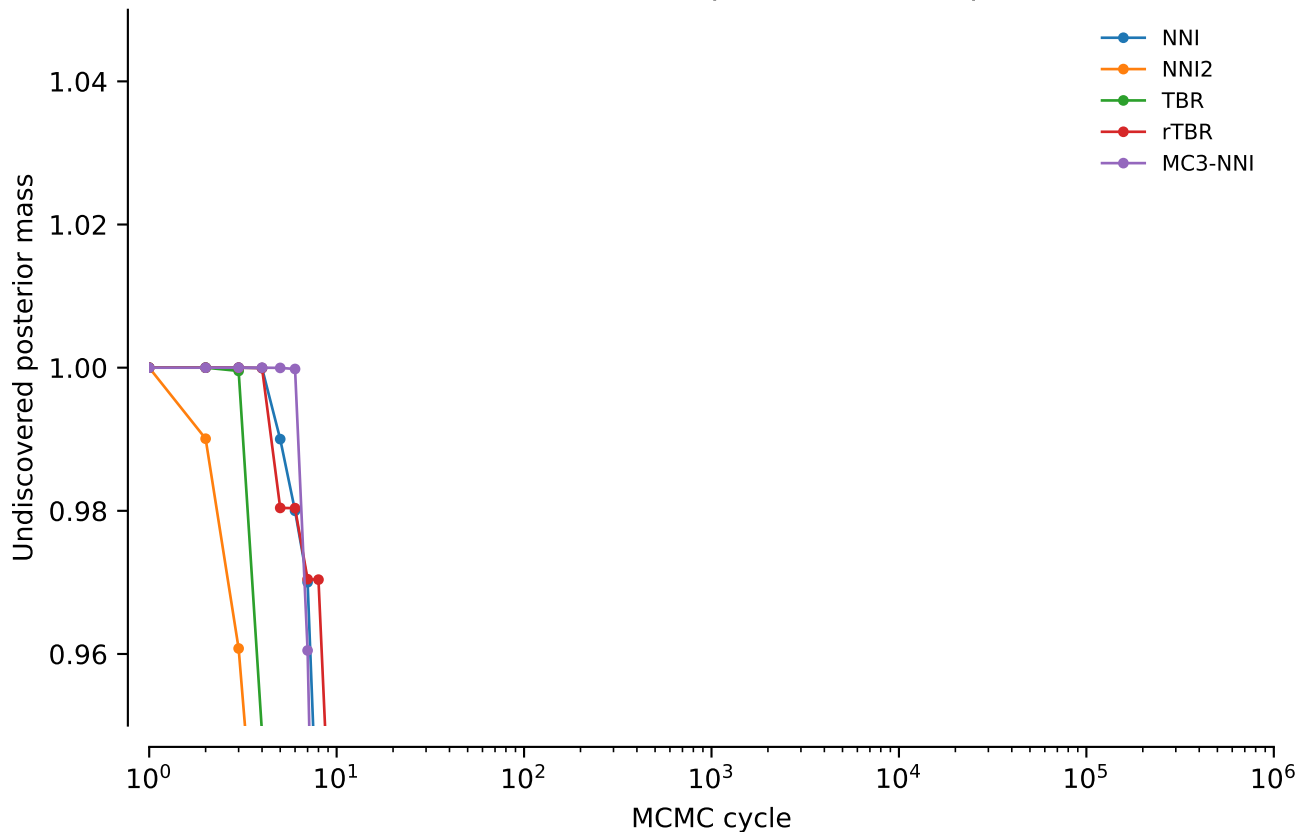
vert.nd2.tw0: Undiscovered posterior mass: power = 0.2
