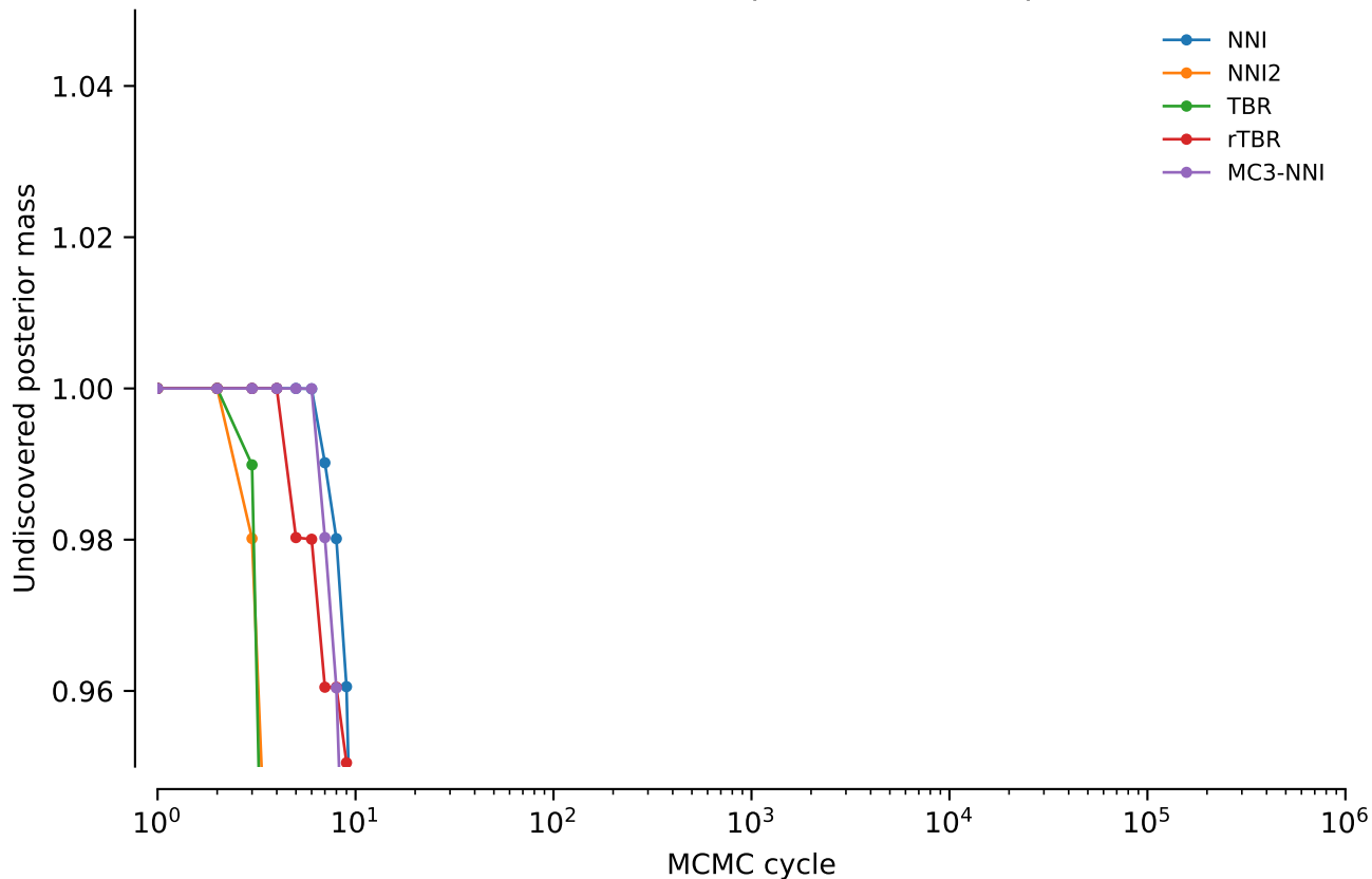
vert.nd2.tw0: Undiscovered posterior mass: power = 0.3
