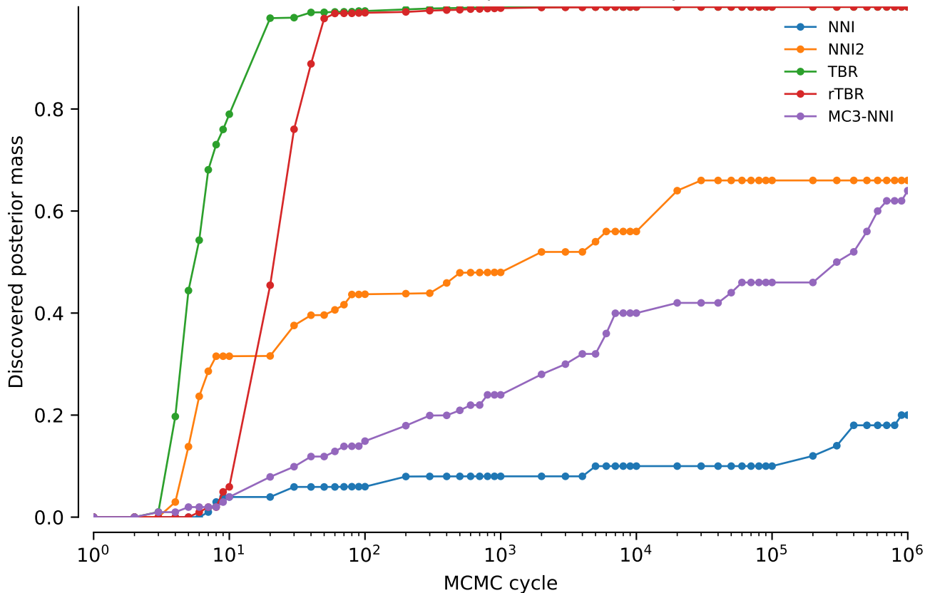
vert.nd2.tw0: Discovered posterior mass: power = 0.4
