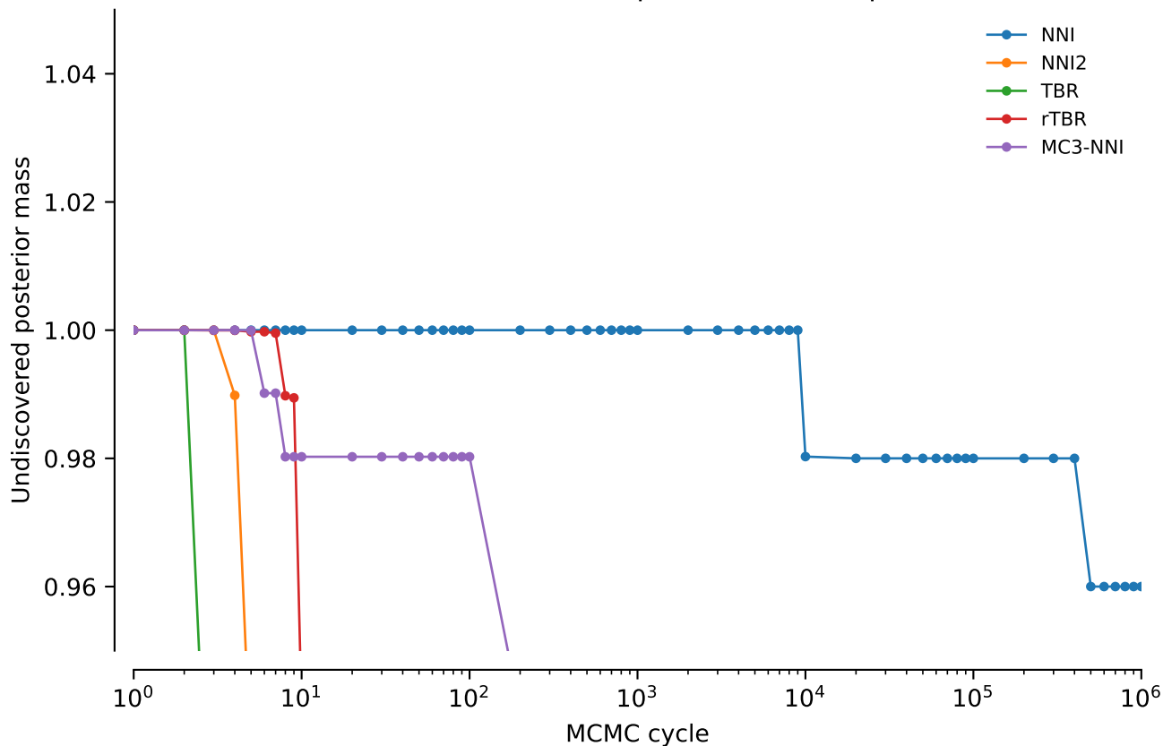
vert.nd2.tw0: Undiscovered posterior mass: power = 0.5
