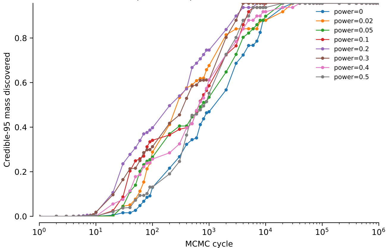
vert.nd2.tw5: NNI power comparison: Credible-95 mass discovered
