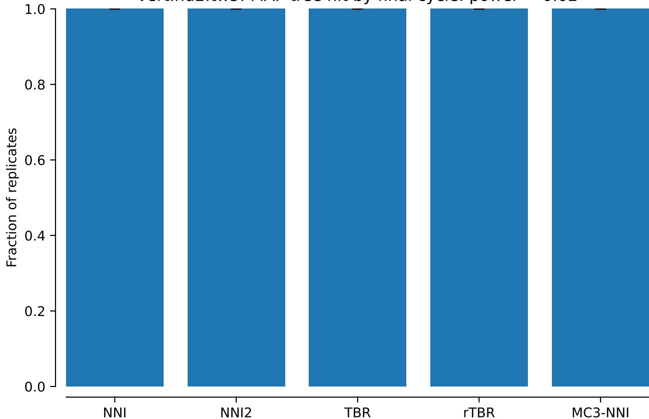
vert.nd2.tw5: MAP tree hit by final cycle: power = 0.02
