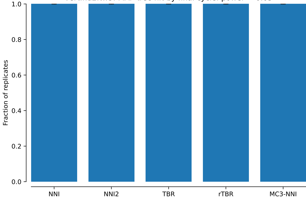
vert.nd2.tw5: MAP tree hit by final cycle: power = 0.05
