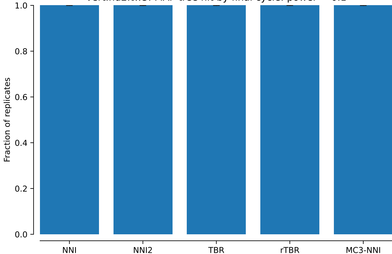
vert.nd2.tw5: MAP tree hit by final cycle: power = 0.1
