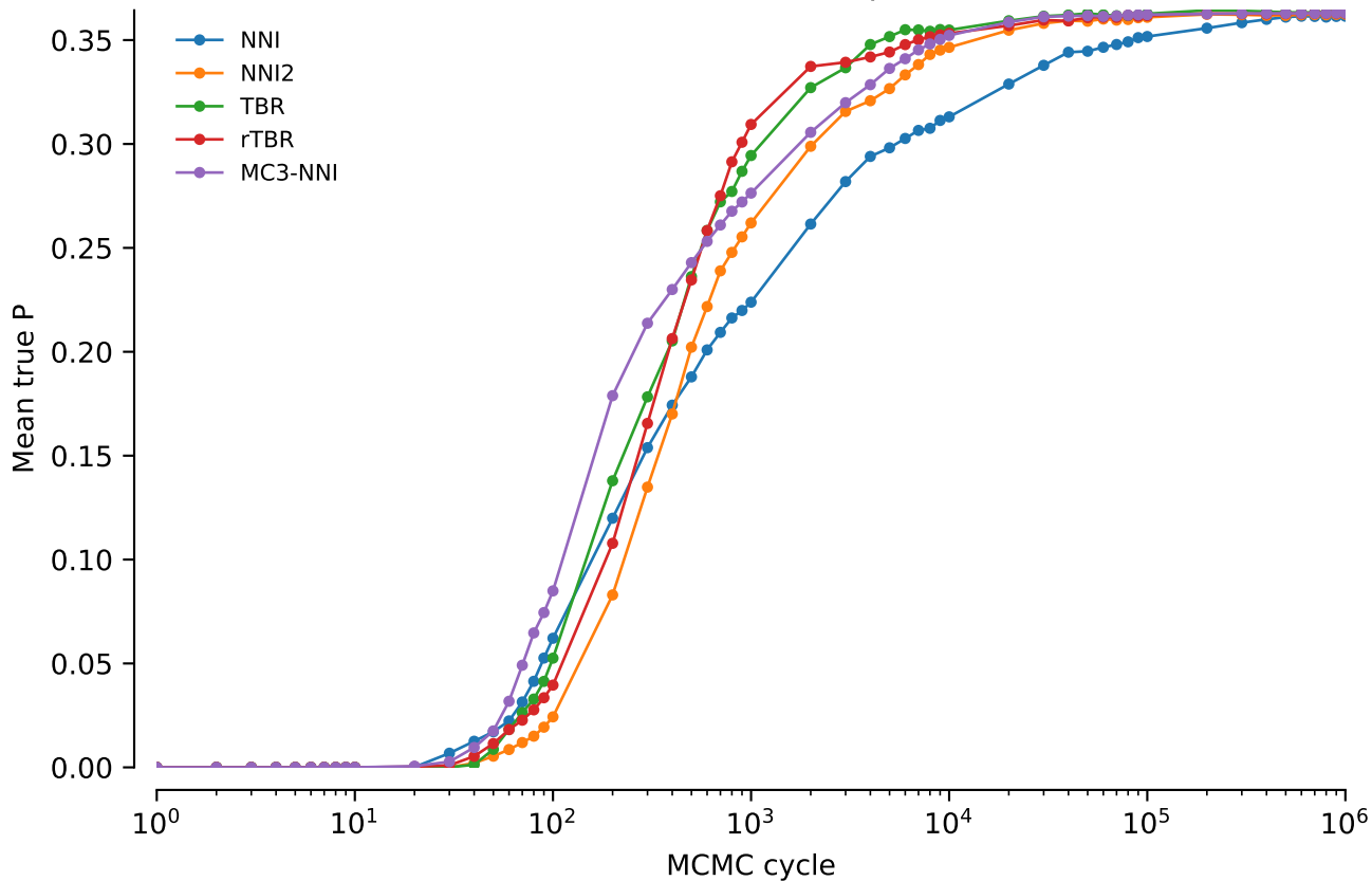
vert.nd2.tw5: Mean true P: power = 0.02
