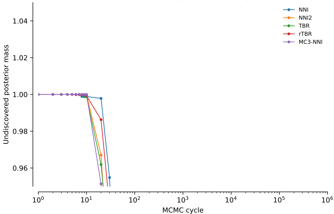
vert.nd2.tw5: Undiscovered posterior mass: power = 0.05
