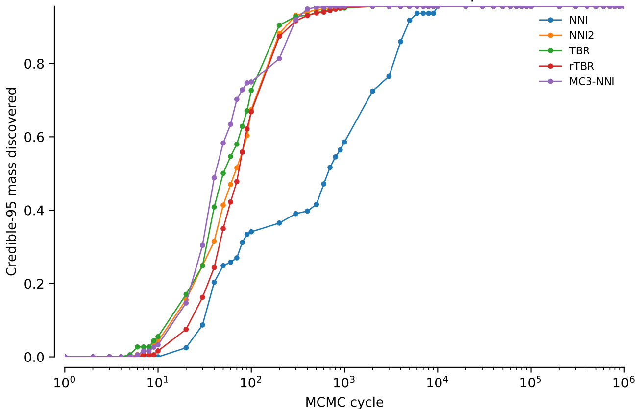
vert.nd2.tw5: Credible-95 mass discovered: power = 0.1
