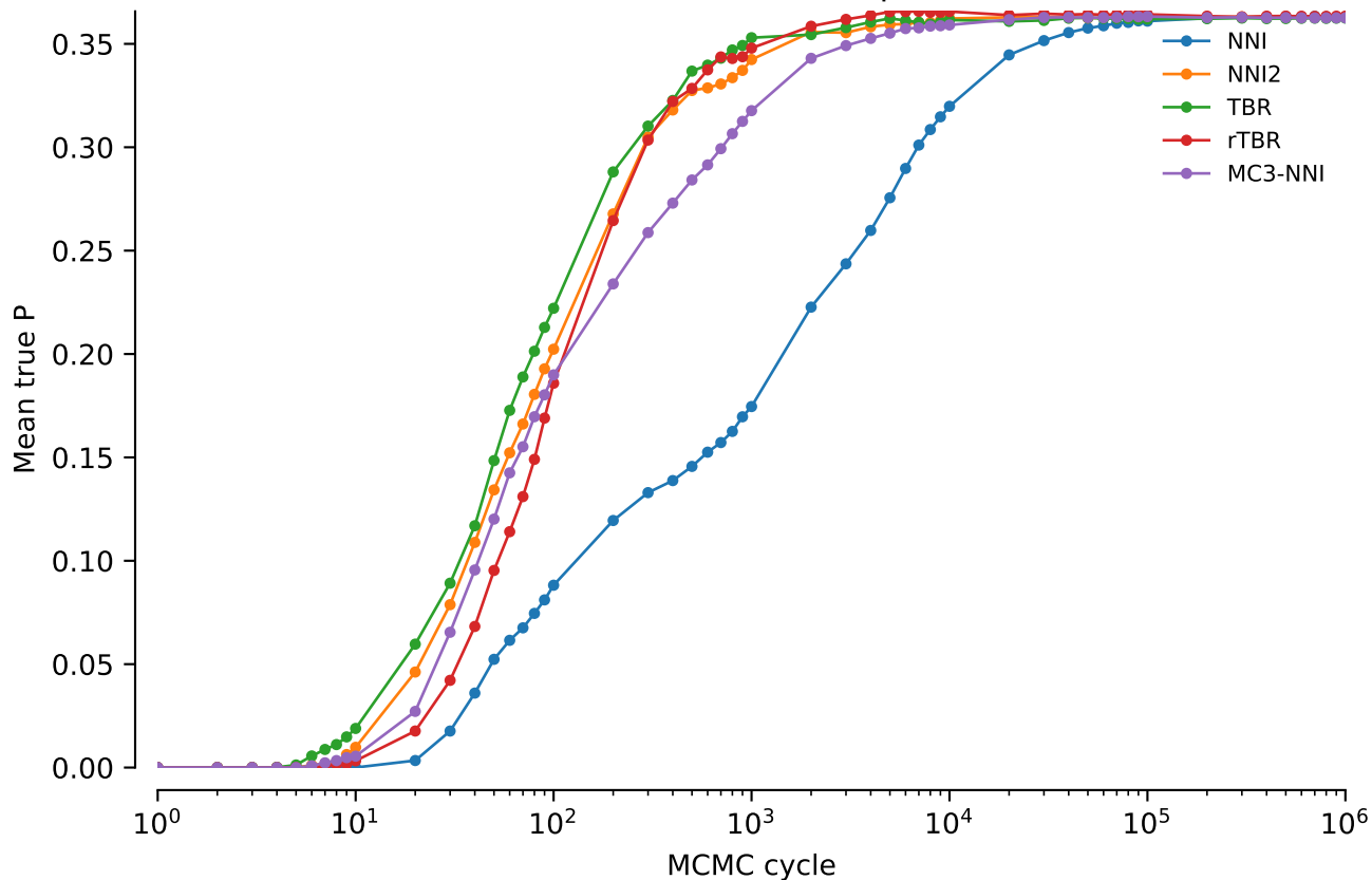
vert.nd2.tw5: Mean true P: power = 0.1
