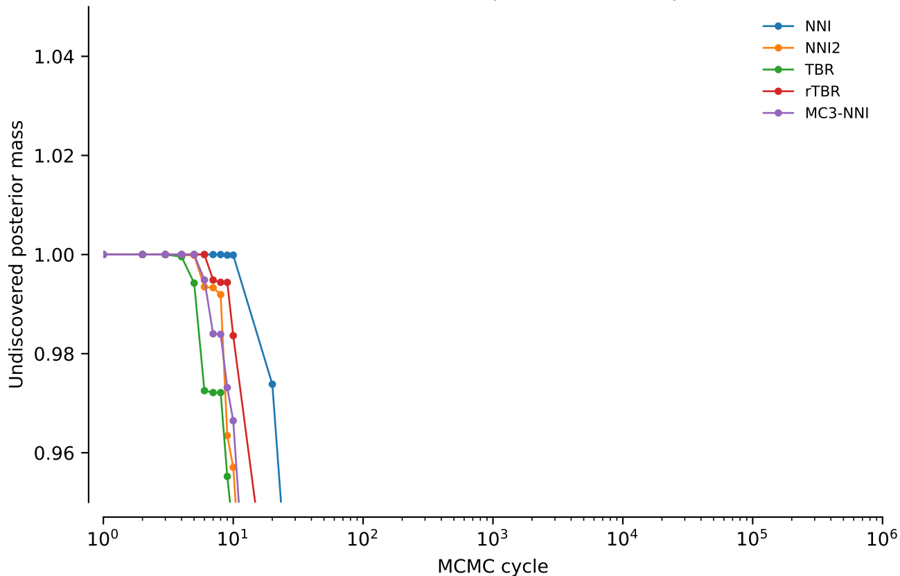
vert.nd2.tw5: Undiscovered posterior mass: power = 0.1
