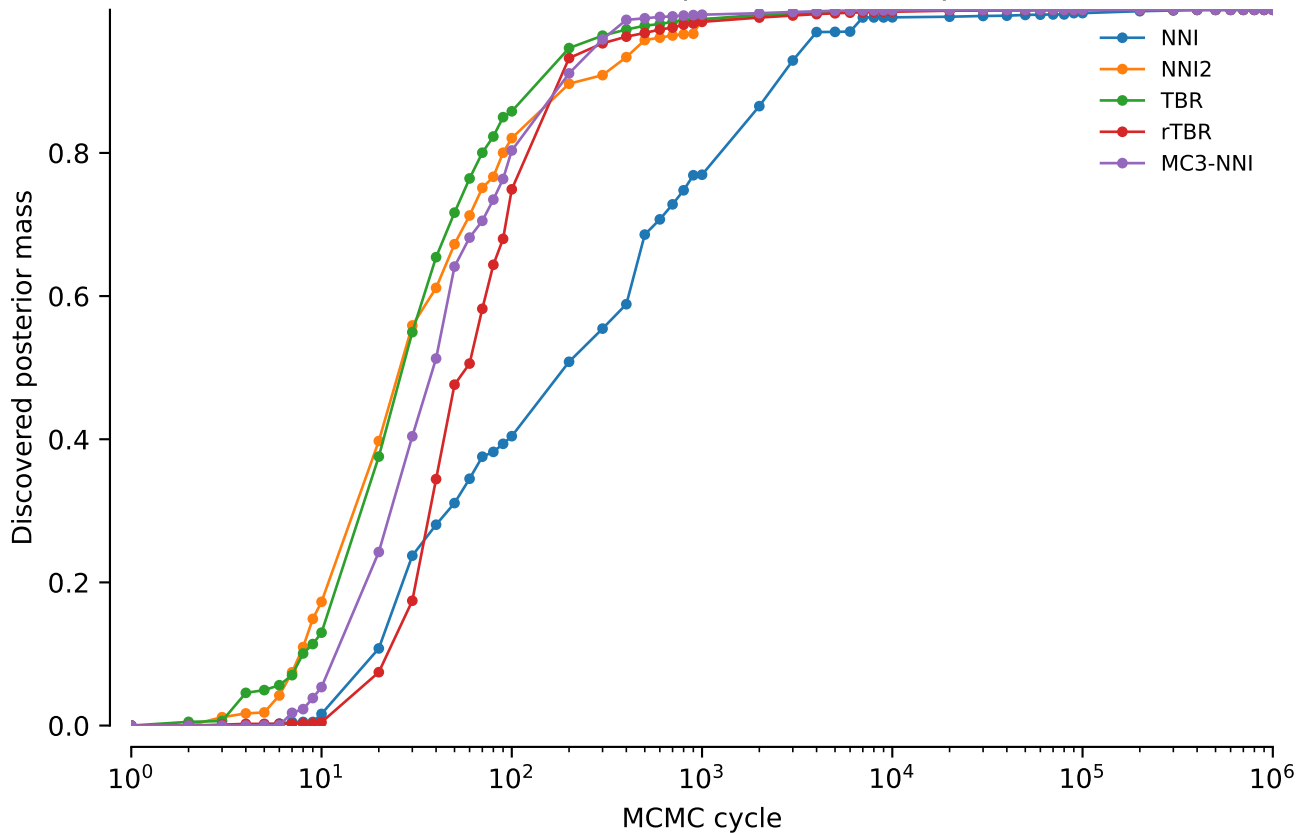
vert.nd2.tw5: Discovered posterior mass: power = 0.2
