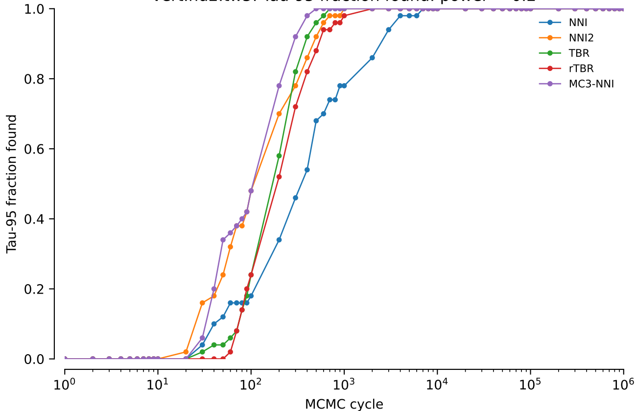
vert.nd2.tw5: Tau-95 fraction found: power = 0.2
