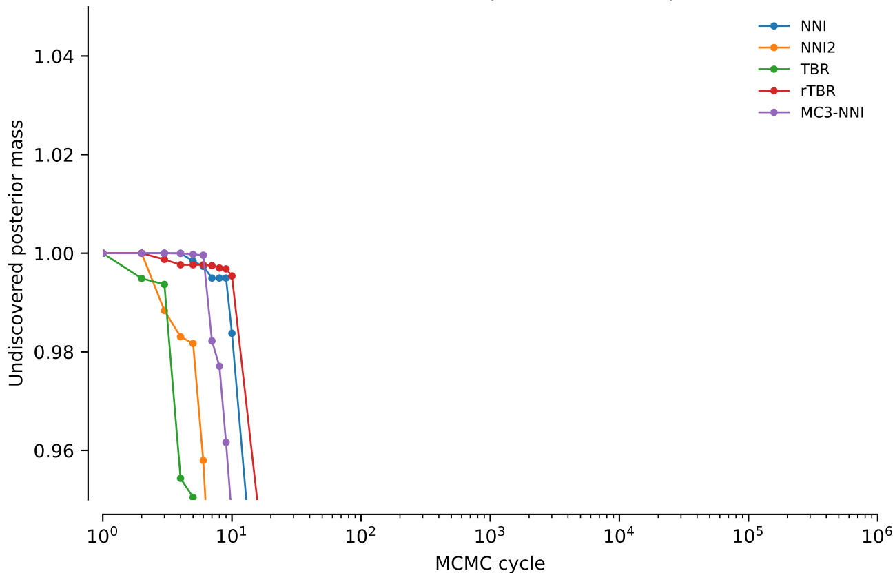
vert.nd2.tw5: Undiscovered posterior mass: power = 0.2
