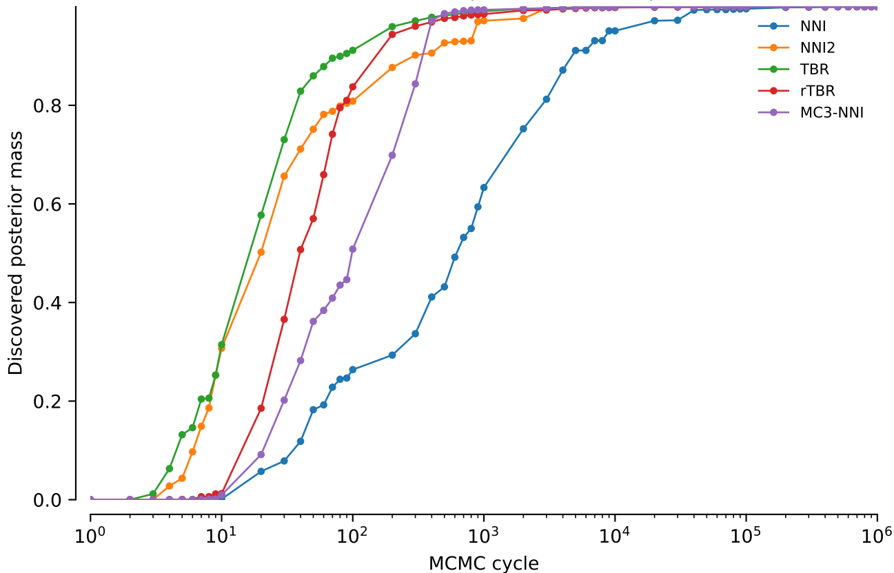
vert.nd2.tw5: Discovered posterior mass: power = 0.4
