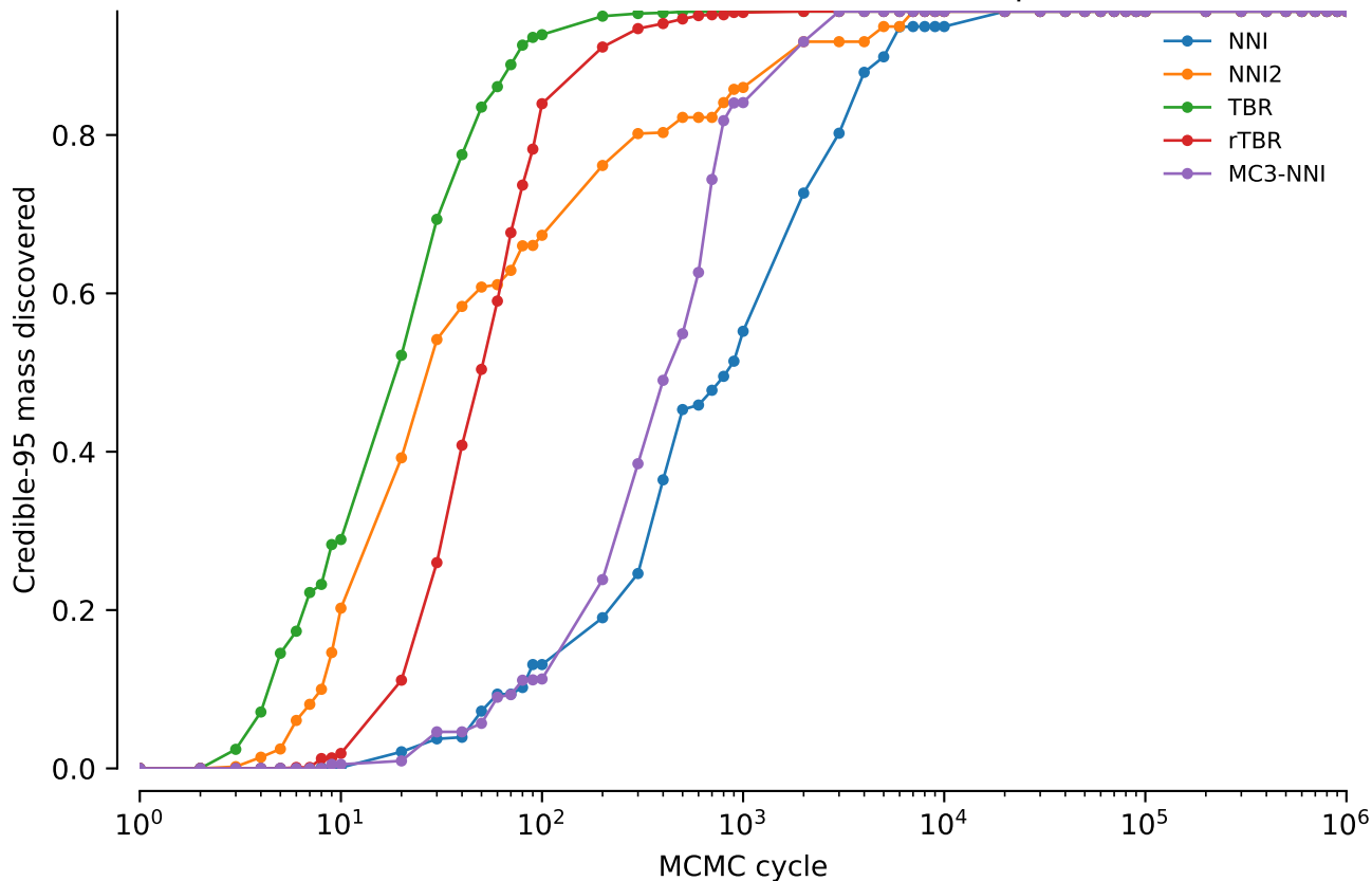
vert.nd2.tw5: Credible-95 mass discovered: power = 0.5
