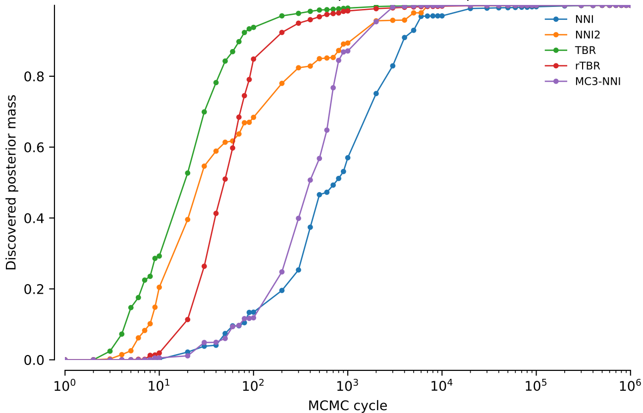
vert.nd2.tw5: Discovered posterior mass: power = 0.5
