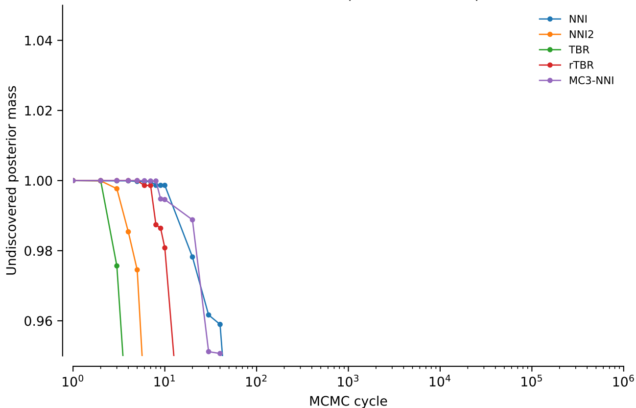
vert.nd2.tw5: Undiscovered posterior mass: power = 0.5
