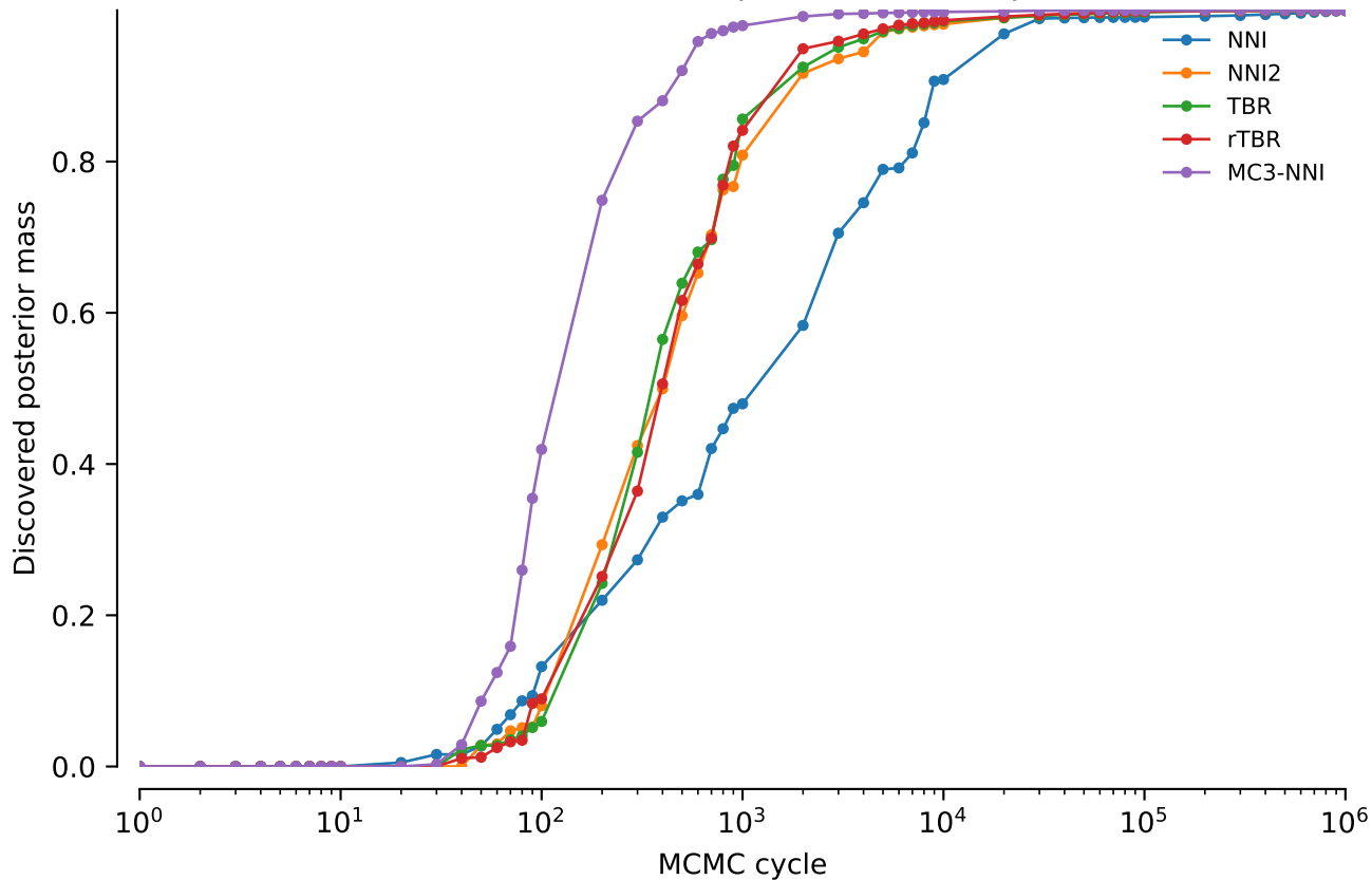
vert.nd2.tw5: Discovered posterior mass: power = 0
