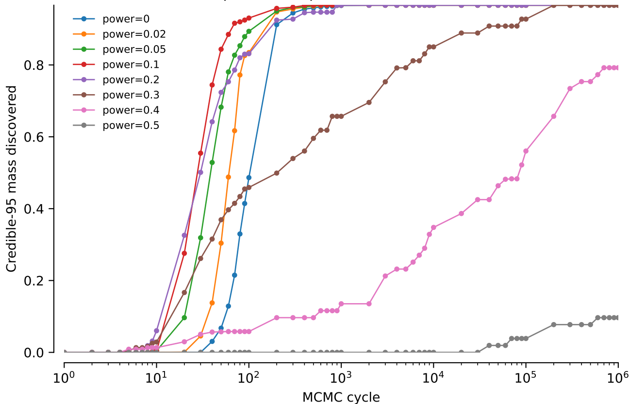
vert.nd3.tw0: NNI power comparison: Credible-95 mass discovered
