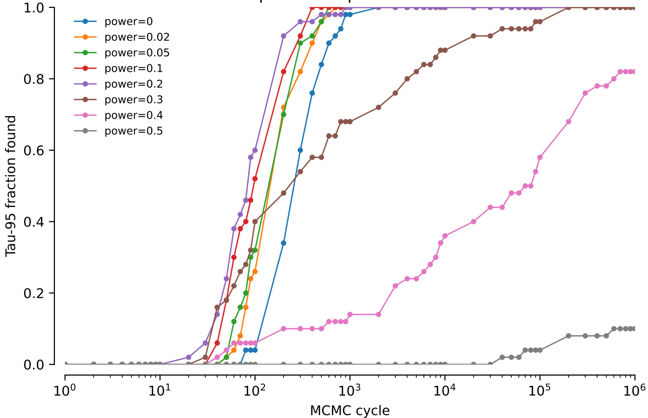
vert.nd3.tw0: NNI power comparison: Tau-95 fraction found
