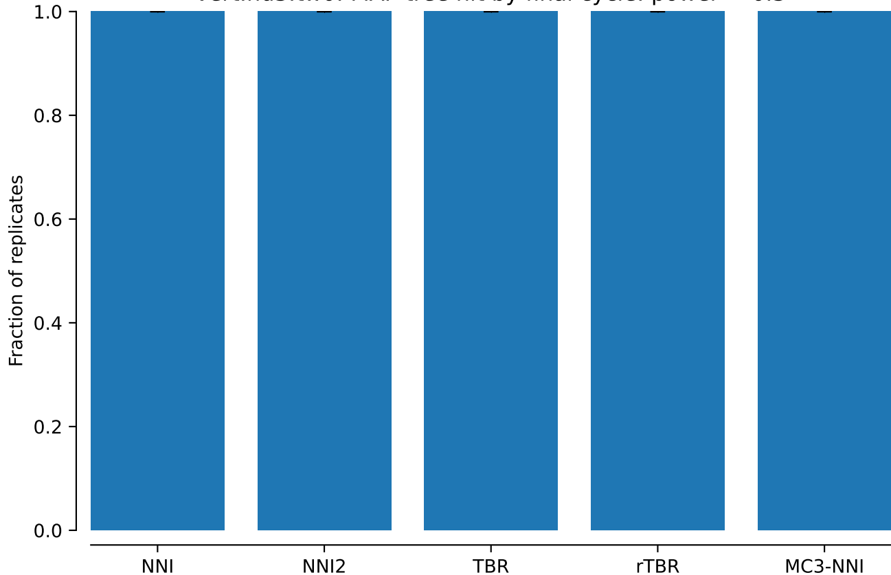
vert.nd3.tw0: MAP tree hit by final cycle: power = 0.3
