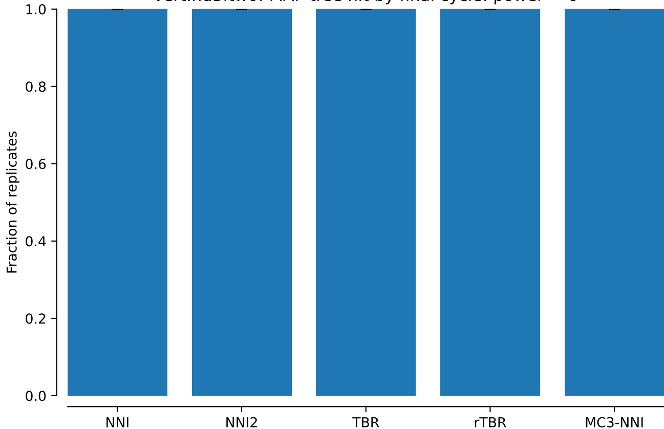
vert.nd3.tw0: MAP tree hit by final cycle: power = 0
