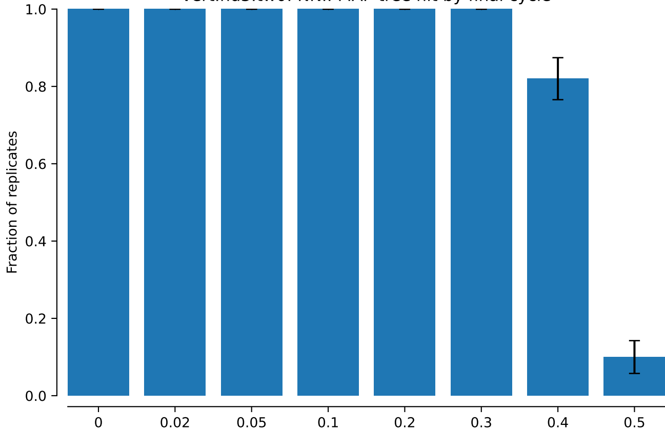
vert.nd3.tw0: NNI: MAP tree hit by final cycle
