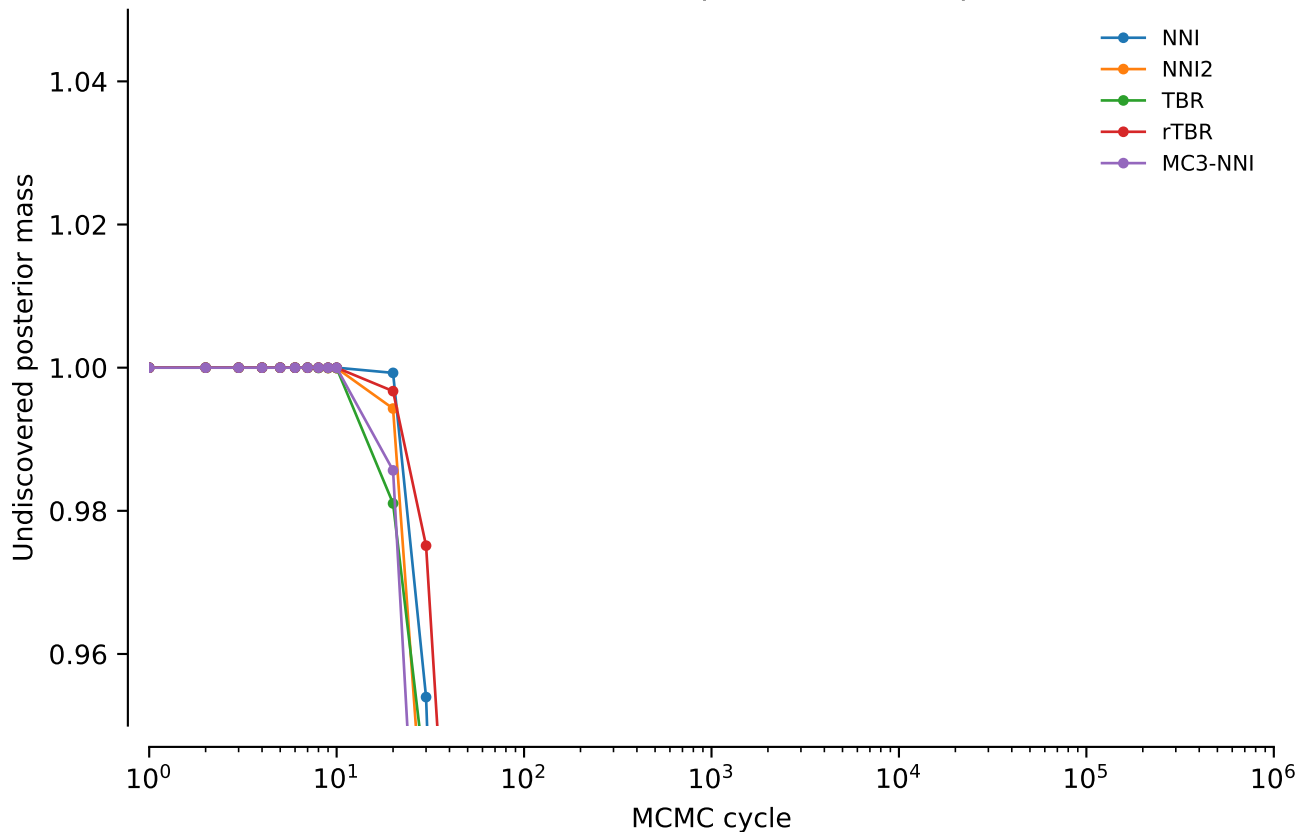
vert.nd3.tw0: Undiscovered posterior mass: power = 0.02
