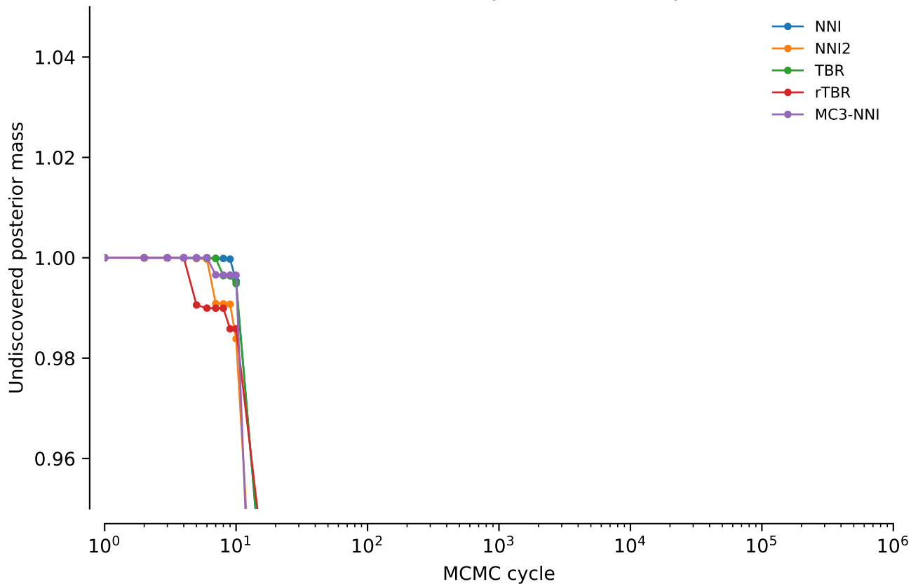
vert.nd3.tw0: Undiscovered posterior mass: power = 0.05
