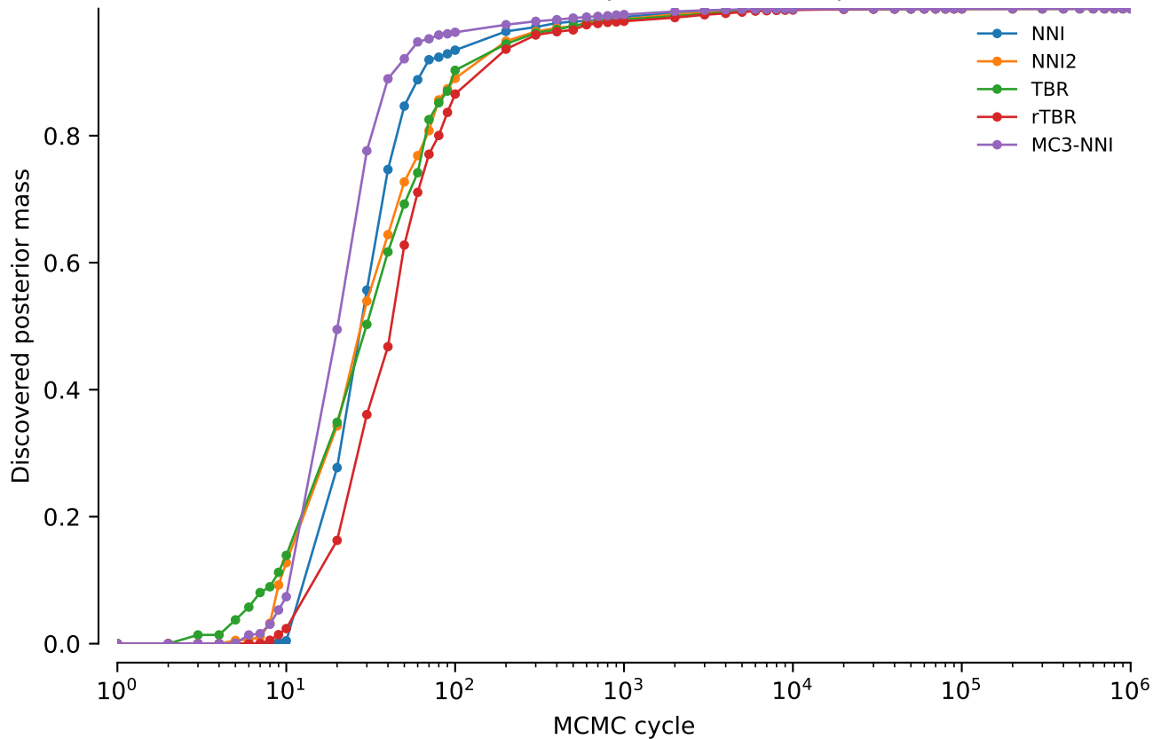
vert.nd3.tw0: Discovered posterior mass: power = 0.1
