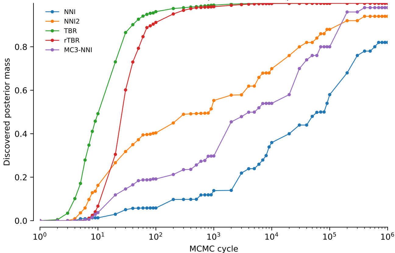
vert.nd3.tw0: Discovered posterior mass: power = 0.4
