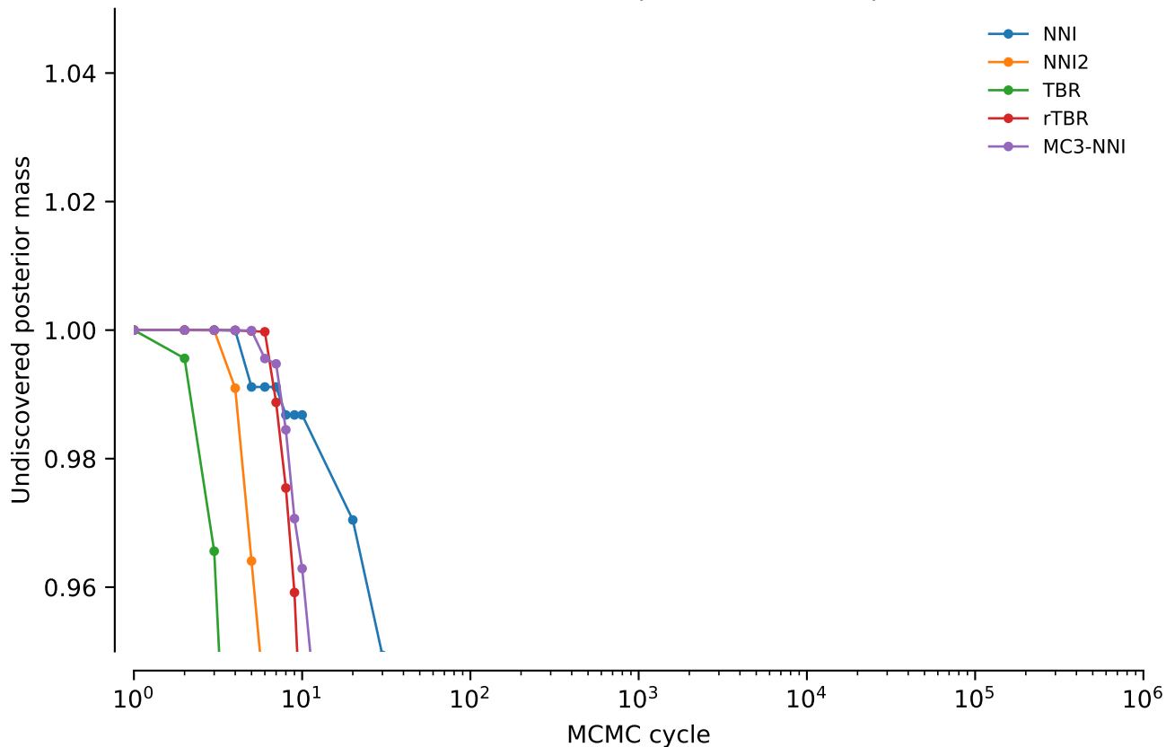
vert.nd3.tw0: Undiscovered posterior mass: power = 0.4
