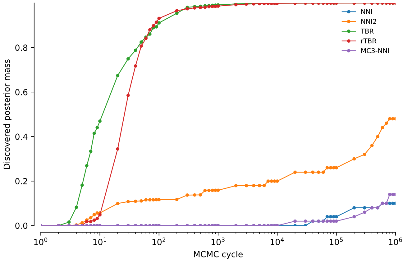
vert.nd3.tw0: Discovered posterior mass: power = 0.5
