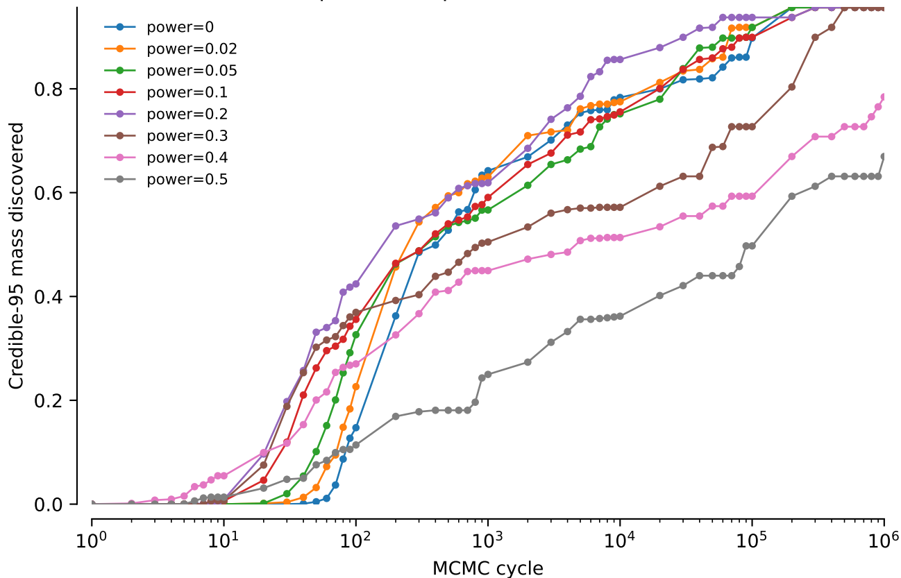
vert.nd3.tw5: NNI power comparison: Credible-95 mass discovered
