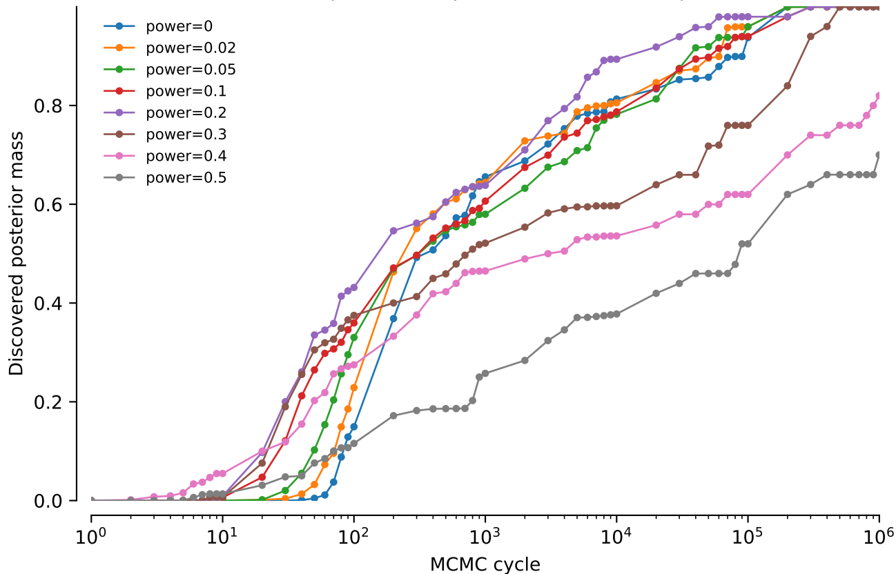
vert.nd3.tw5: NNI power comparison: Discovered posterior mass
