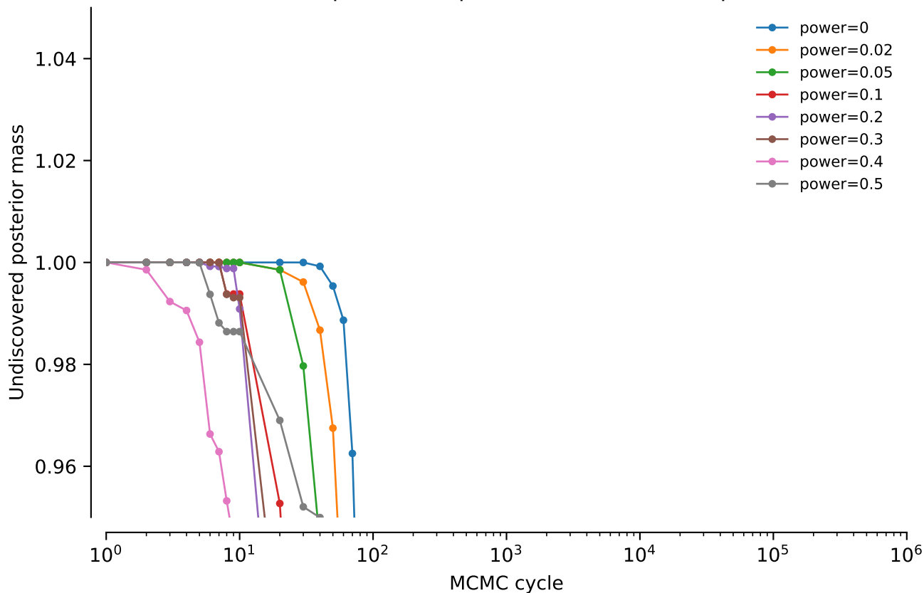
vert.nd3.tw5: NNI power comparison: Undiscovered posterior mass
