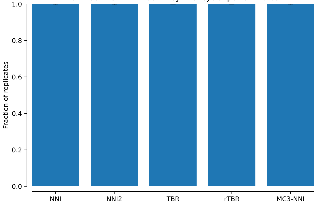
vert.nd3.tw5: MAP tree hit by final cycle: power = 0.05
