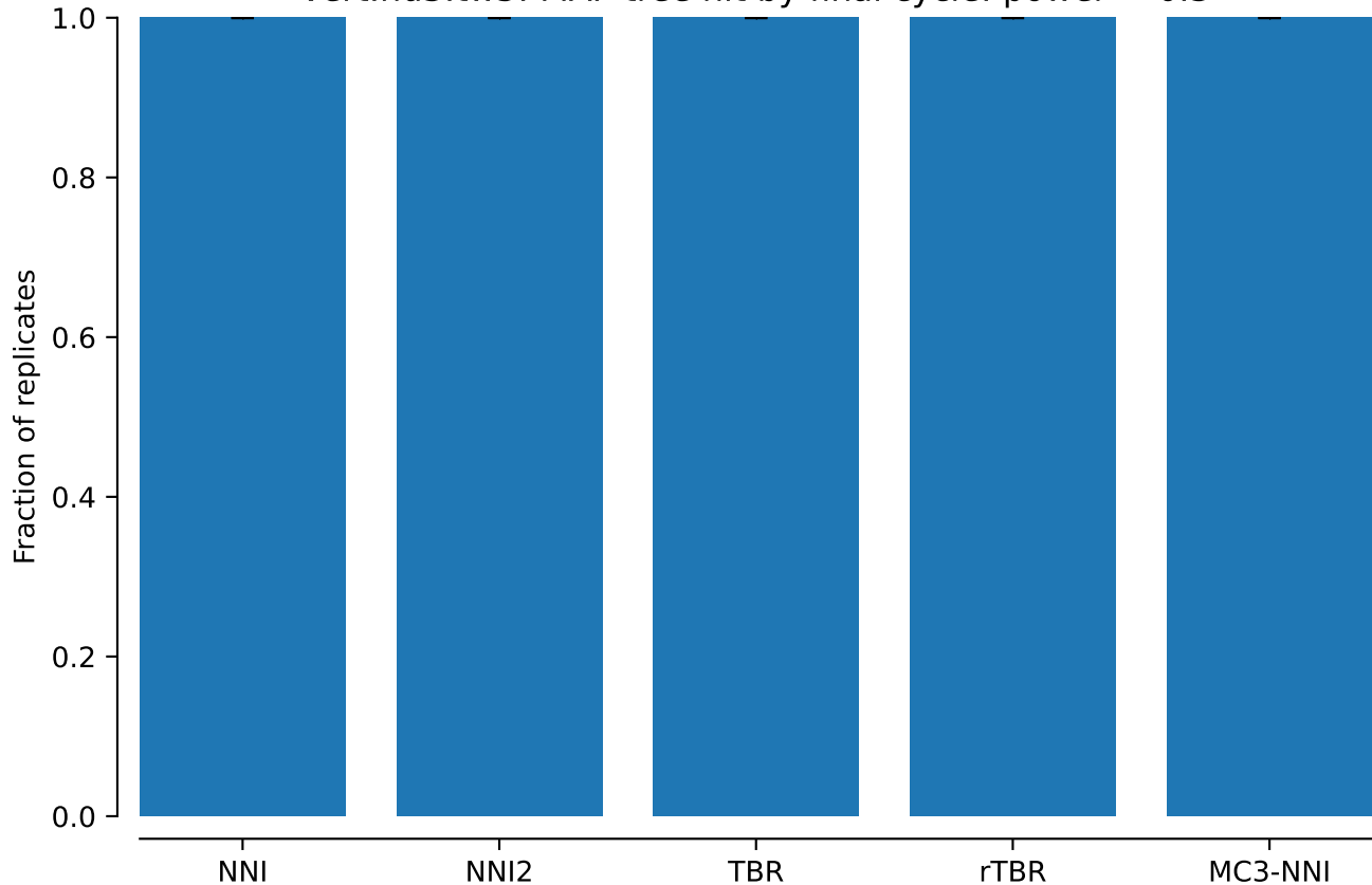
vert.nd3.tw5: MAP tree hit by final cycle: power = 0.3
