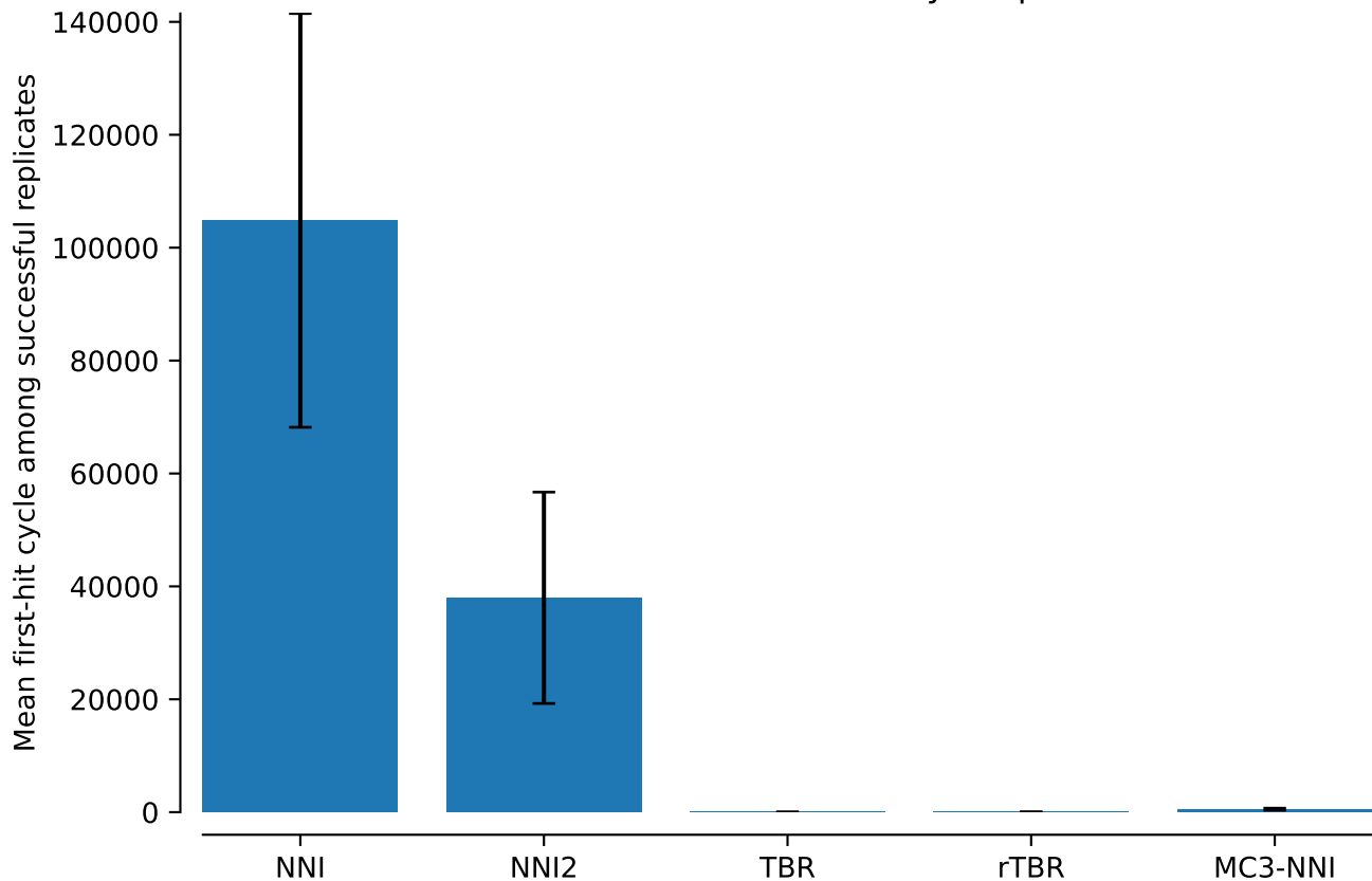
vert.nd3.tw5: Mean MAP first-hit cycle: power = 0.4
