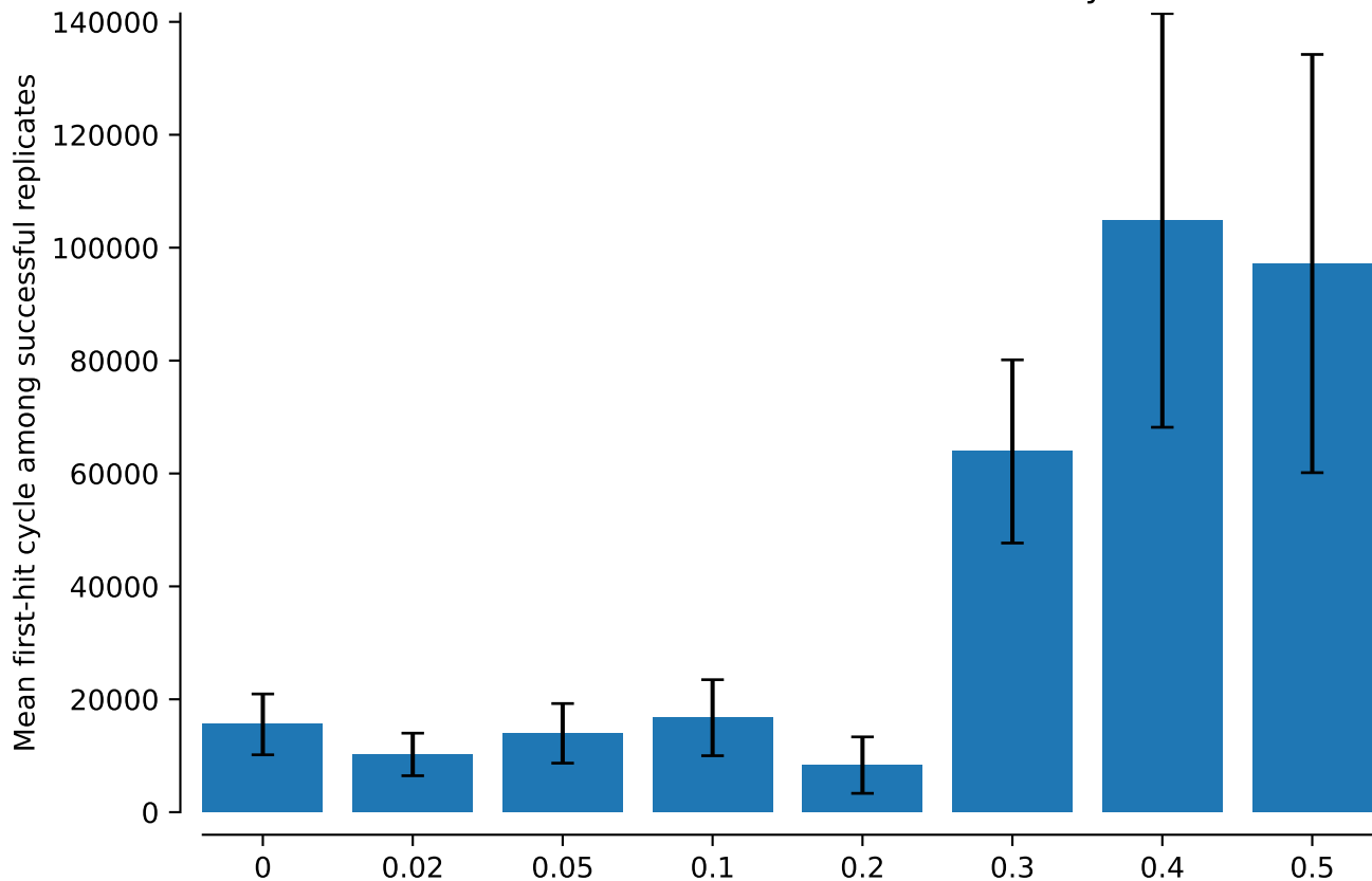
vert.nd3.tw5: NNI: mean MAP first-hit cycle
