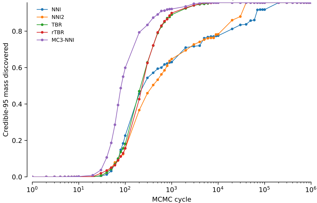
vert.nd3.tw5: Credible-95 mass discovered: power = 0.02
