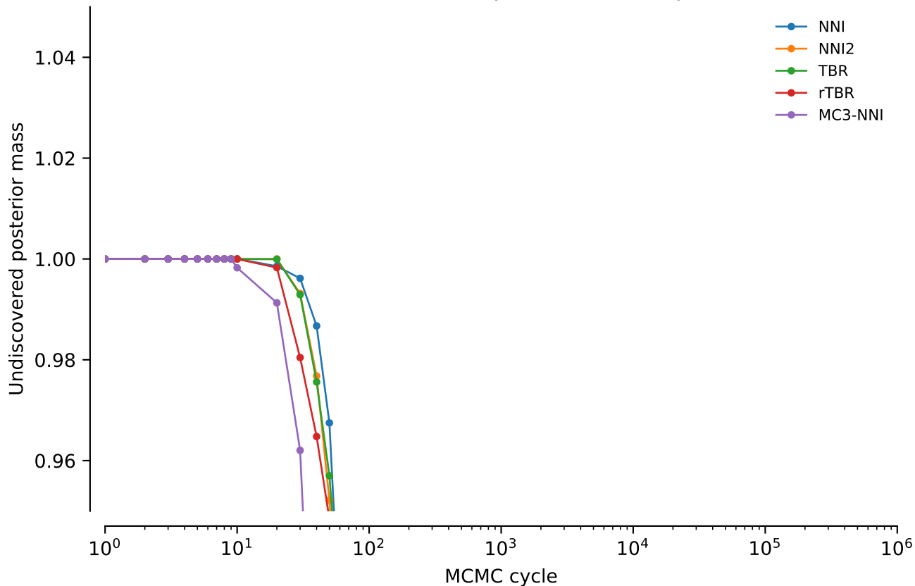
vert.nd3.tw5: Undiscovered posterior mass: power = 0.02
