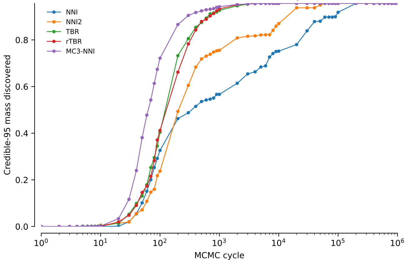
vert.nd3.tw5: Credible-95 mass discovered: power = 0.05
