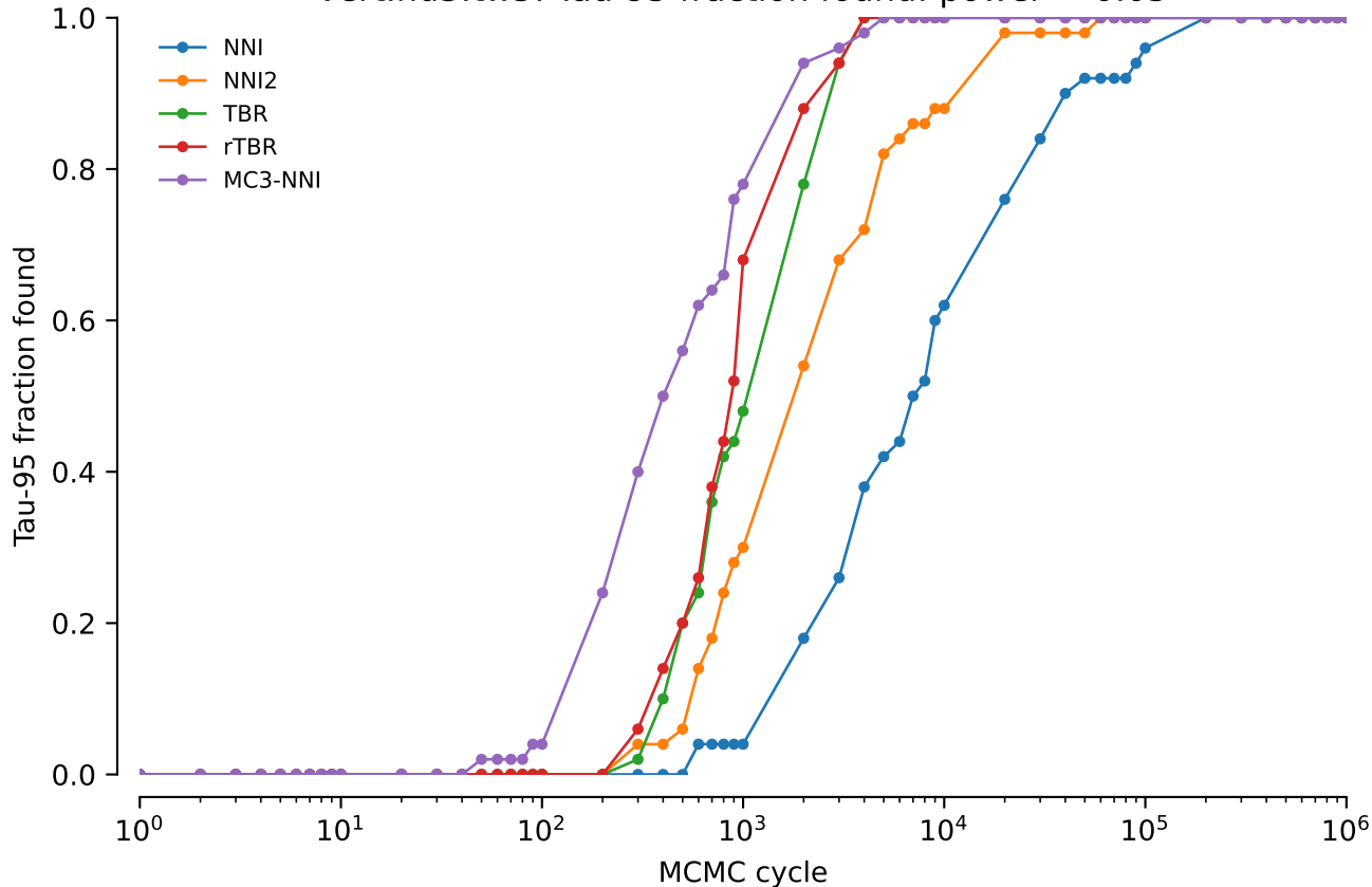
vert.nd3.tw5: Tau-95 fraction found: power = 0.05
