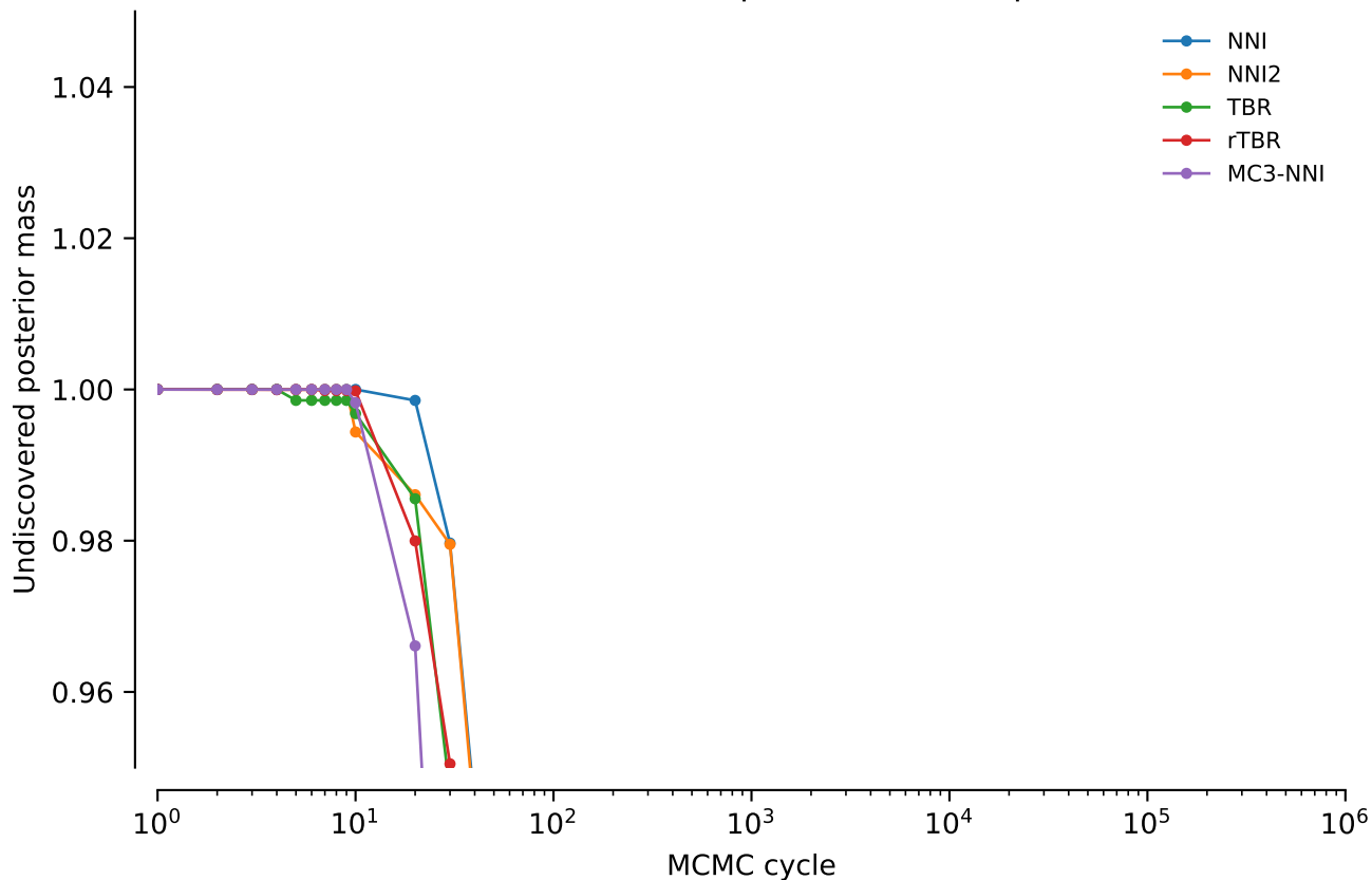
vert.nd3.tw5: Undiscovered posterior mass: power = 0.05
