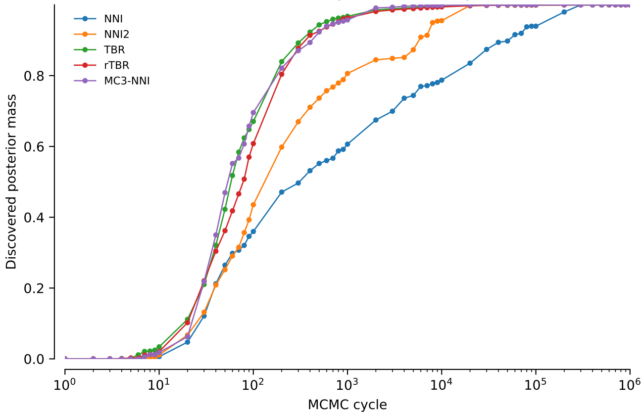
vert.nd3.tw5: Discovered posterior mass: power = 0.1
