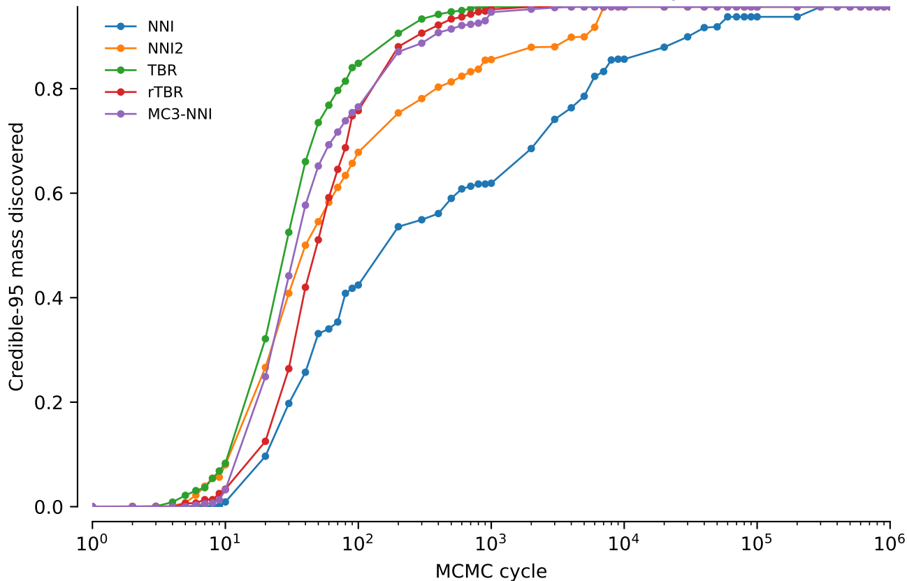
vert.nd3.tw5: Credible-95 mass discovered: power = 0.2
