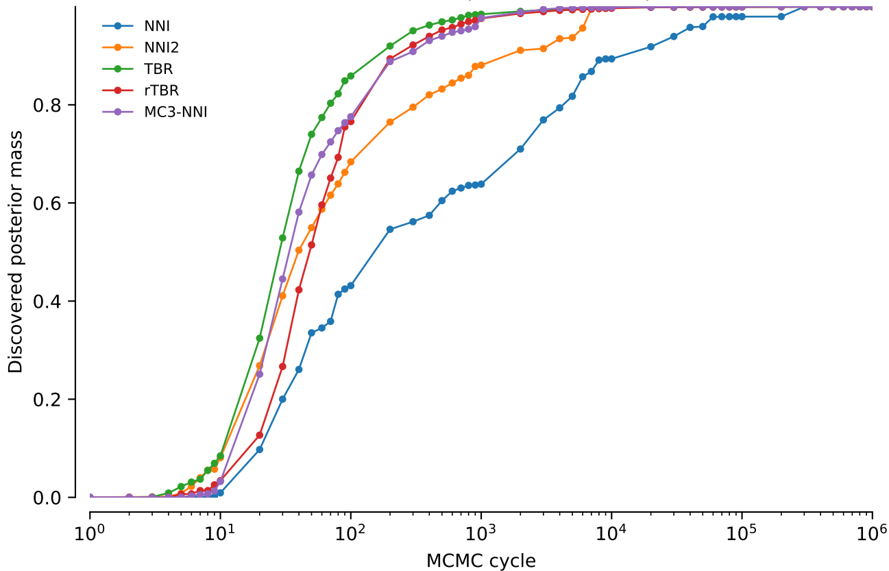
vert.nd3.tw5: Discovered posterior mass: power = 0.2
